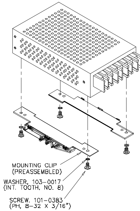
FIGURE 3. INSTALLATION OF KIT ON ERD 60W POWER SUPPLY
