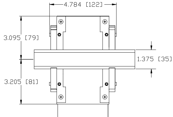
FIGURE 4. ERD 60W POWER SUPPLY WITH KIT INSTALLED, OUTLINE DIMENSIONS
