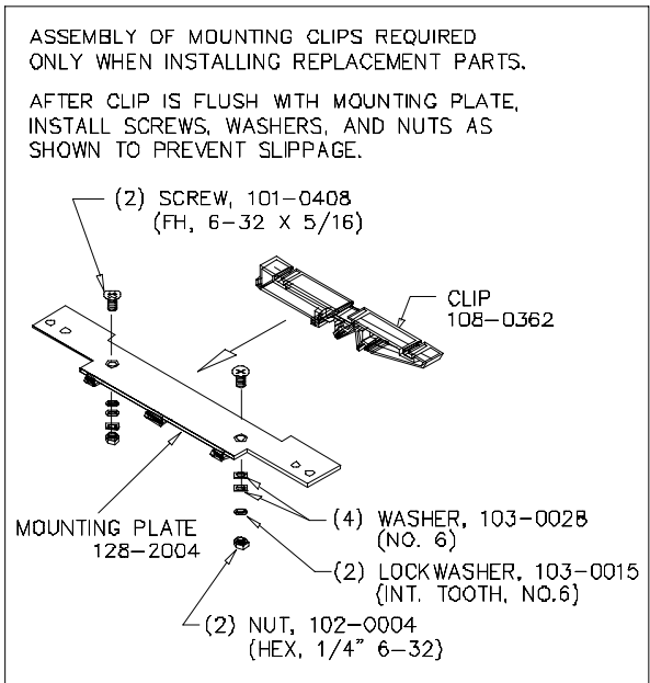
FIGURE 3. INSTALLATION OF KIT ON ERD 60W POWER SUPPLY
